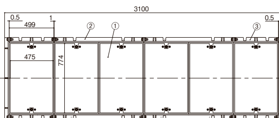
MICC-W6 (6連蓋) (枠開口750×3000)
